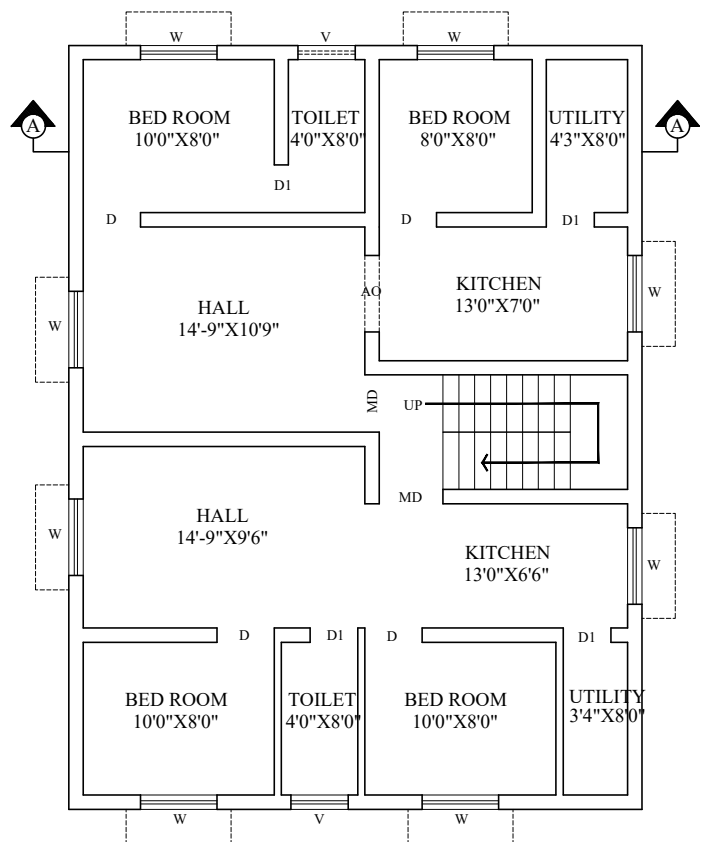
TYPICAL FLOOR PLAN FIRST & SECOND FLOOR PLAN
