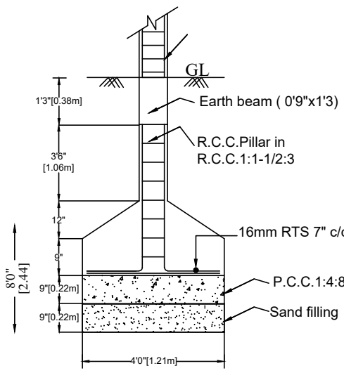
FOUNDATION DETAILS
