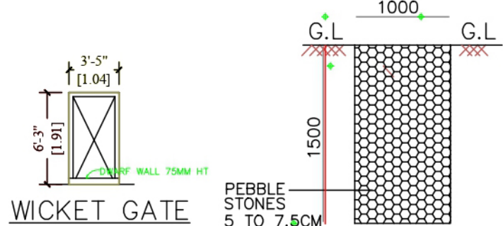
SECTION OF PEBBLE TRENCH SCALE : 1: = 100
