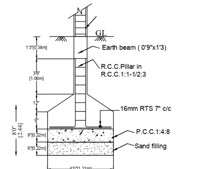
FOUNDATION DETAILS
