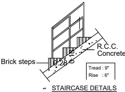
STAIRCASE DETAILS
