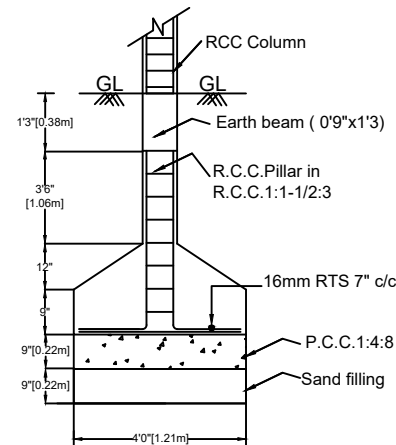
FOUNDATION DETAILS
