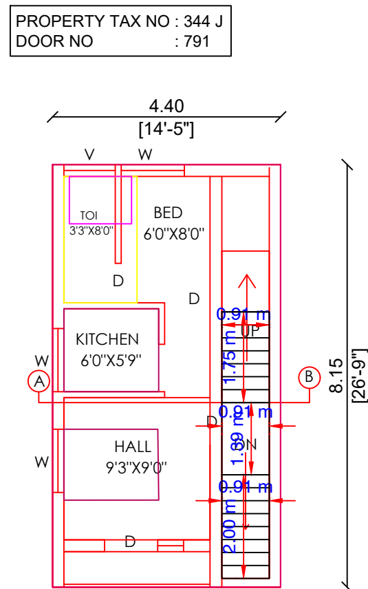
PRO.FIRSTFLOOR PLAN
