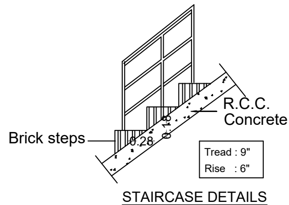
STAIRCASE DETAILS
