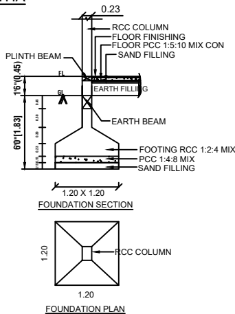
FOUNDATION SECTION
