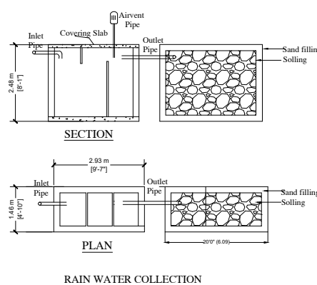
RAIN WATER COLLECTION
