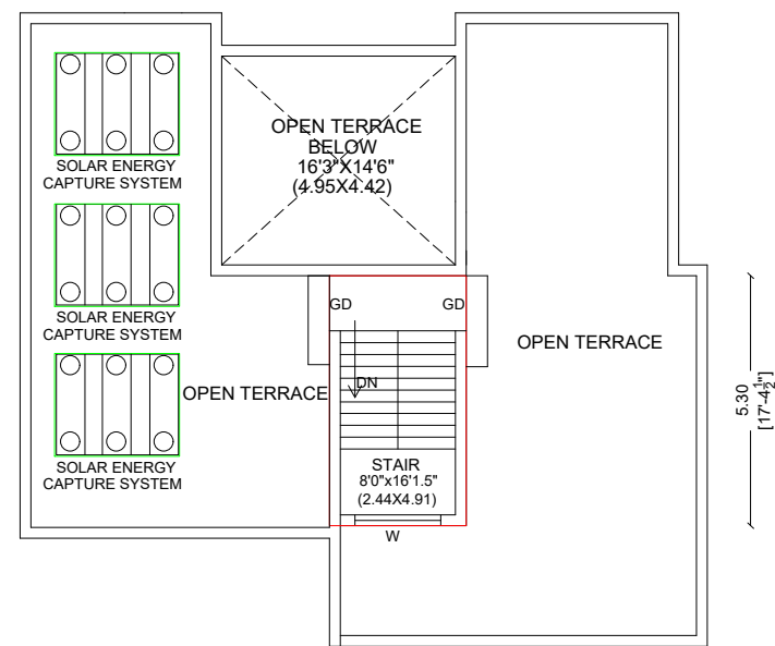
PRO.OPEN TERRACE
