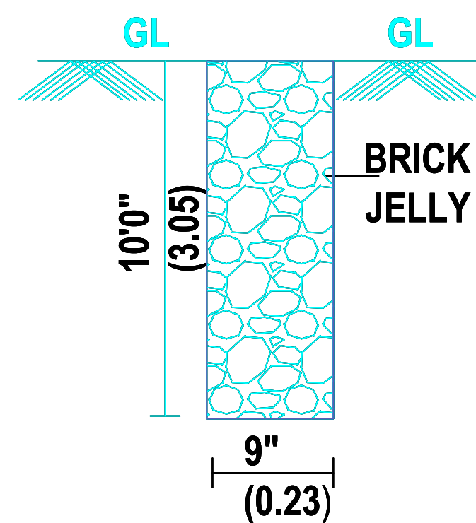
PERCOLATION PIT
