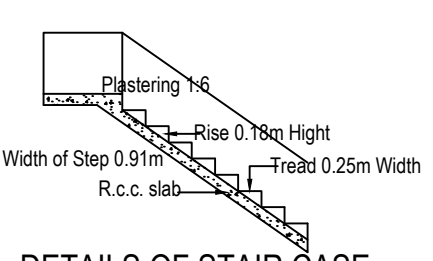
DETAILS OF STAIR CASE
