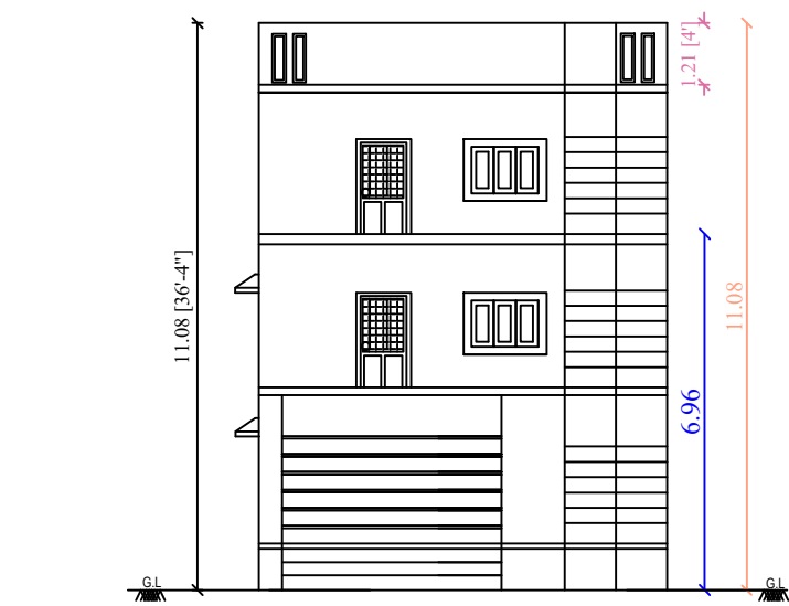
FRONT ELEVATION
