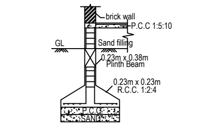
FOUNDATION DETAILS
