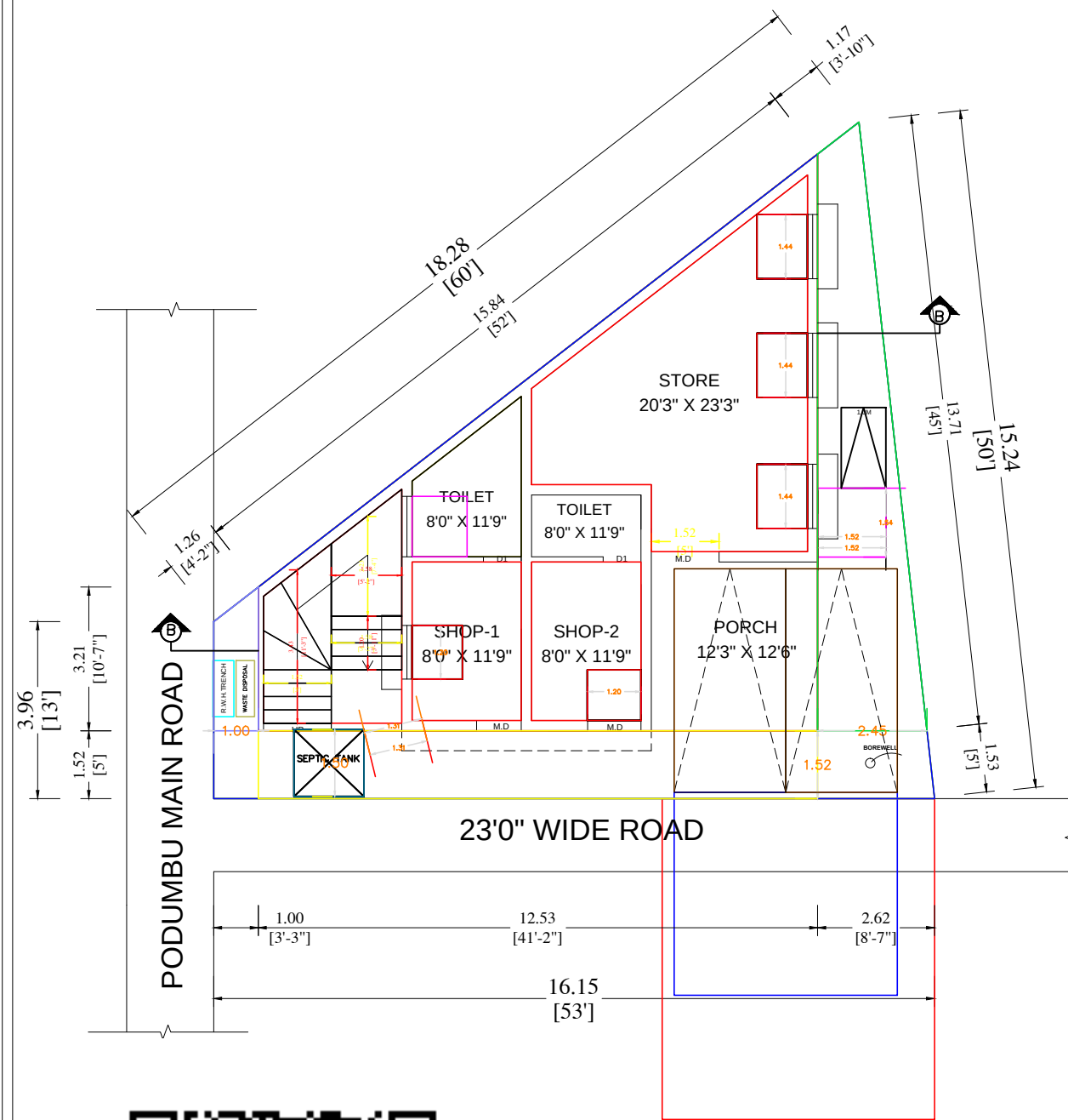
ND FLOOR PLAN PROPOSED
