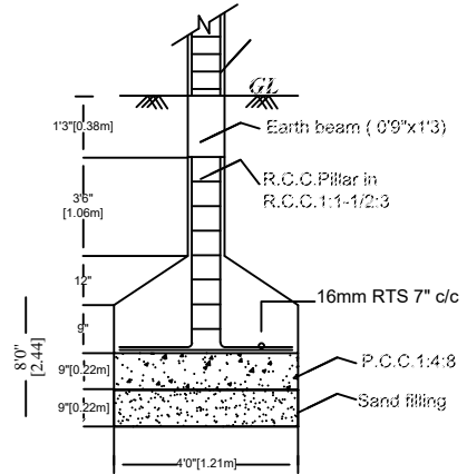
FOUNDATION DETAILS
