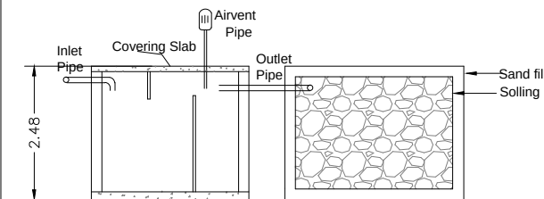
SECTION
