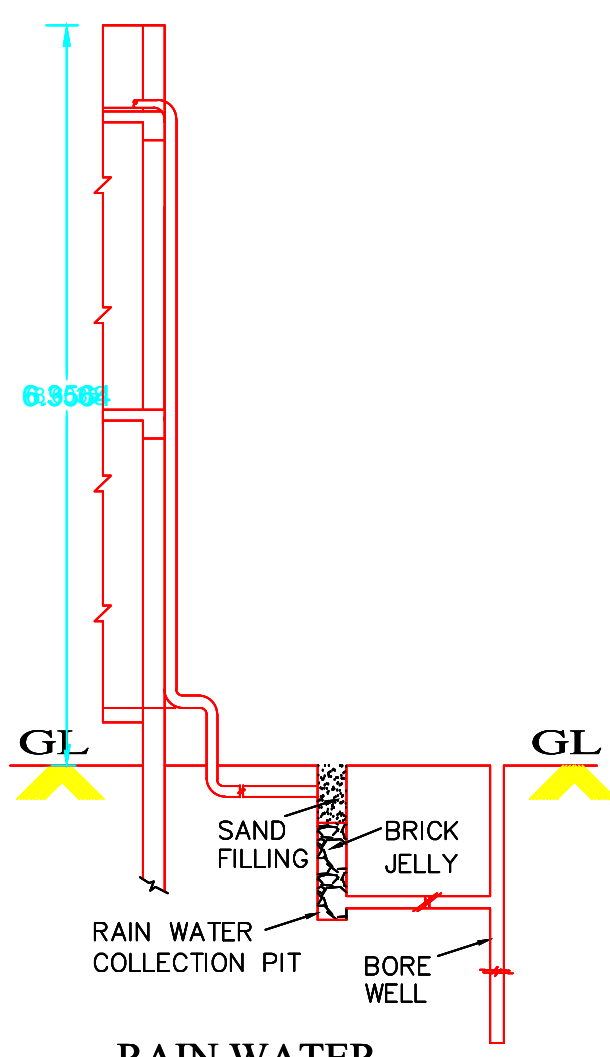
RAIN WATER HARVESTING SYSTEM RWH_CAPACITY_L=1000LTRS
