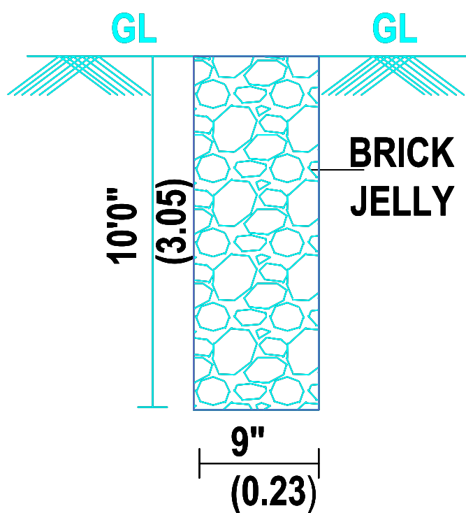
PERCOLATION PIT
