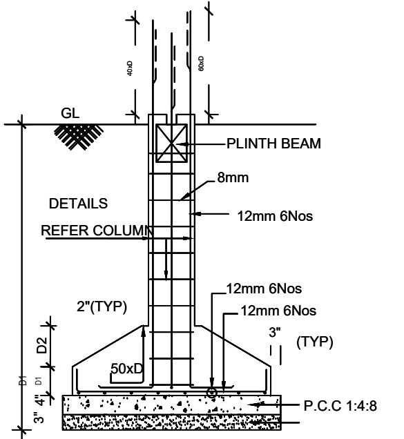
FOUNDATION DETAILS
