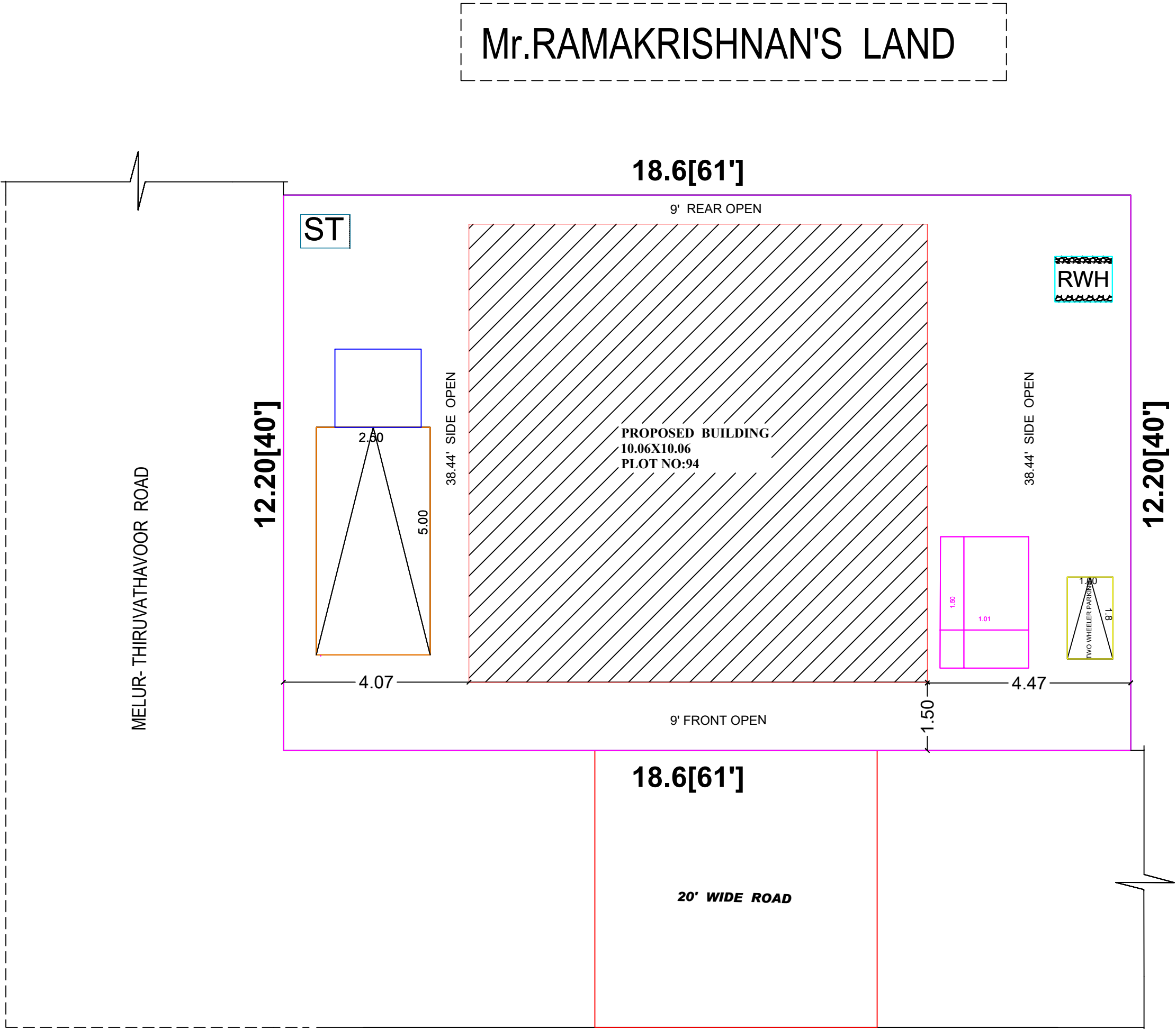
SITE PLAN
