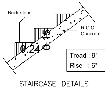
STAIRCASE DETAILS
