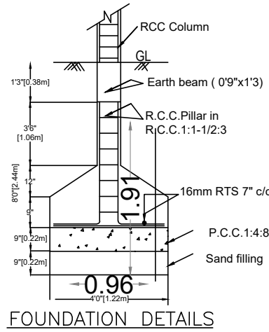
FOUNDATION DETAILS
