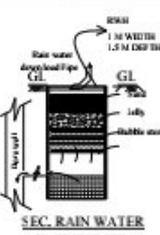
SEC. RAIN WATER HARVEST PIT
