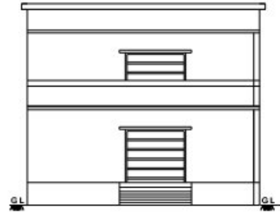
FRONT ELEVATION
