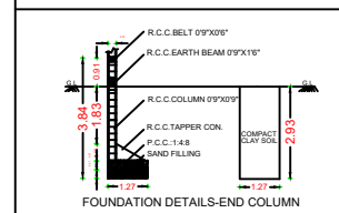
FOUNDATION DETAILS-END COLUMN
