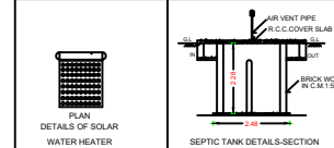
SEPTIC TANK DETAILS-SECTION
