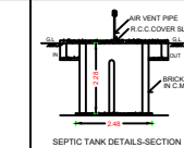
SEPTIC TANK DETAILS-SECTION
