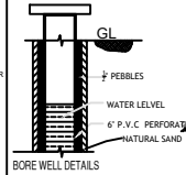
BORE WELL DETAILS
