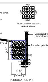
PERCOLATION PIT
