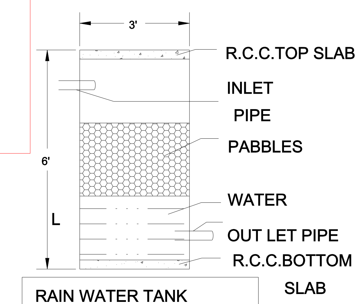
RAIN WATER TANK
