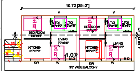
PRO.FIRST FLOOR PLAN
