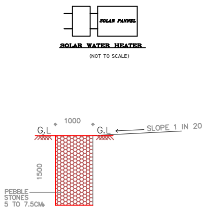
SECTION OF PEBBLE TRENCH SCALE : 1" = 100
