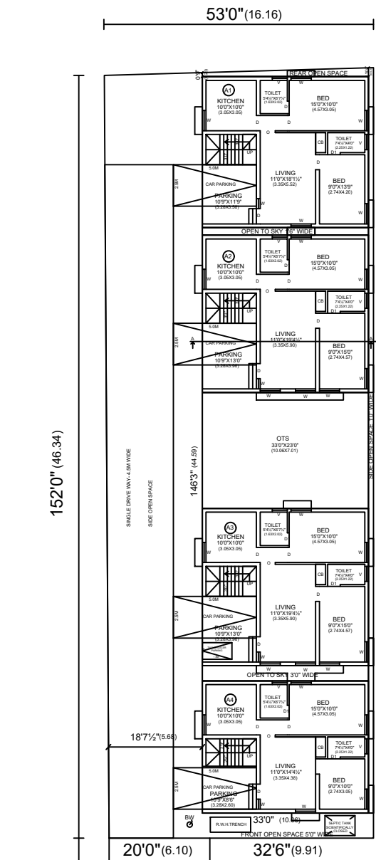
GROUND FLOOR PLAN (PROPOSED)
