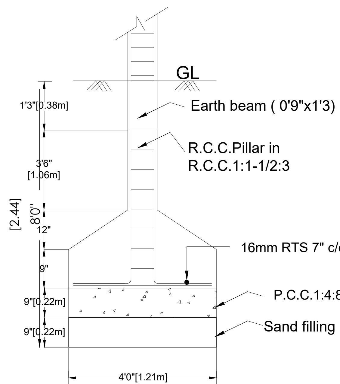
FOUNDATION DETAILS
