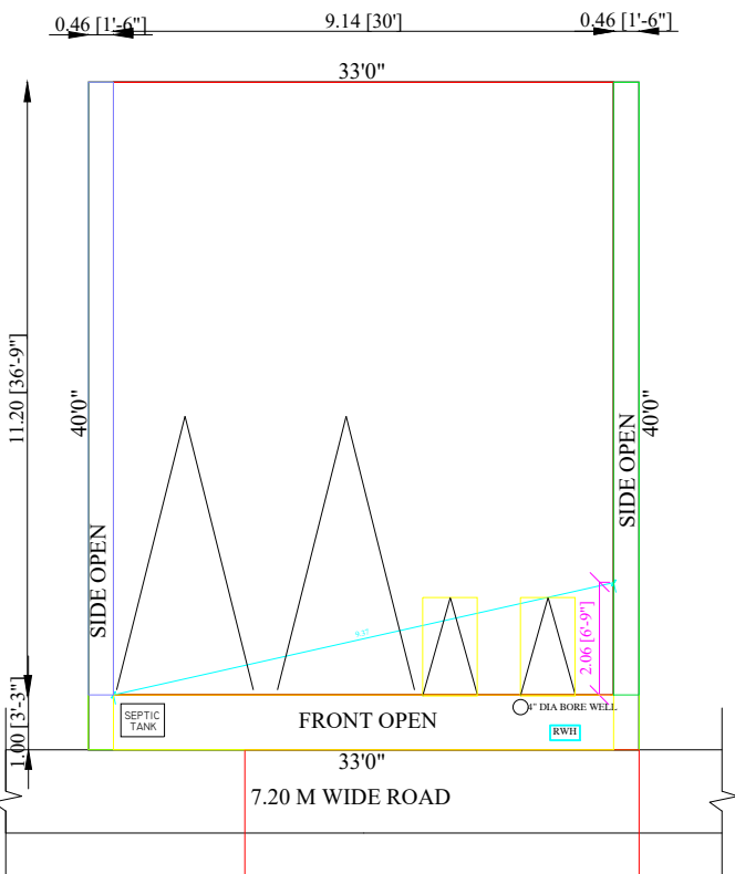
SITE PLAN
