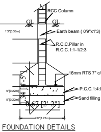
FOUNDATION DETAILS
