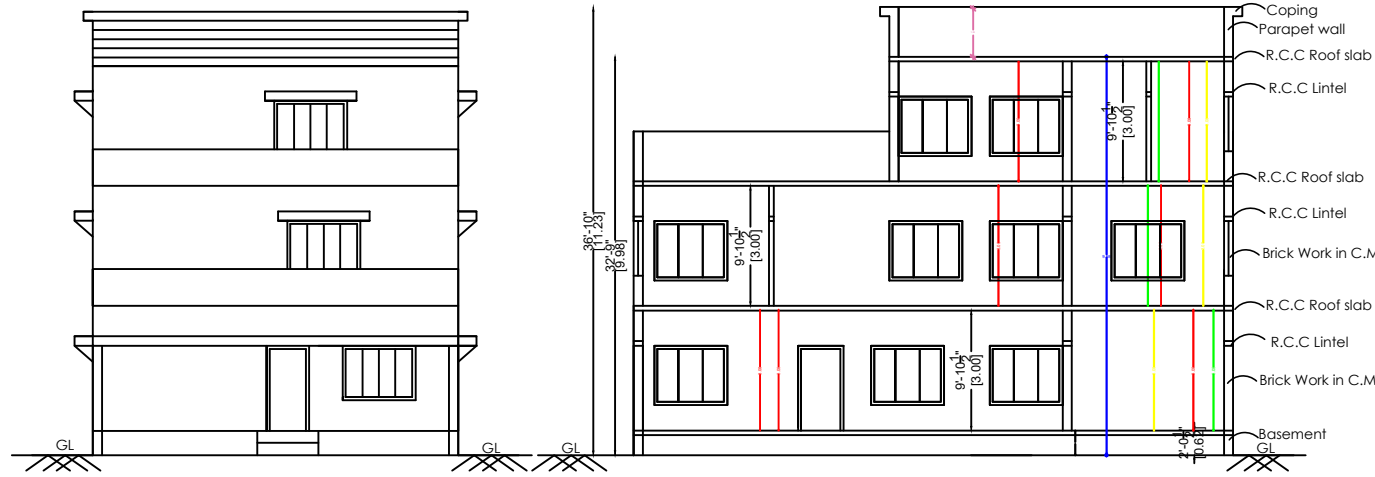
FRONT ELEVATION
