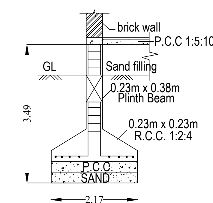
FOUNDATION DETAILS
