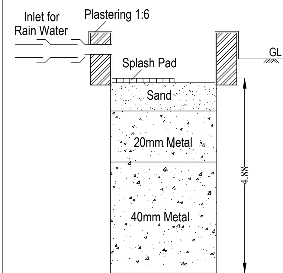
← 2.67 → RAIN WATER PERCOLATION PIT
