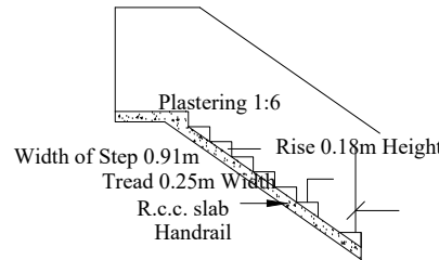
DETAILS OF STAIR CASE
