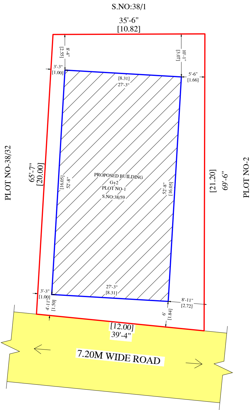
SITE PLAN
