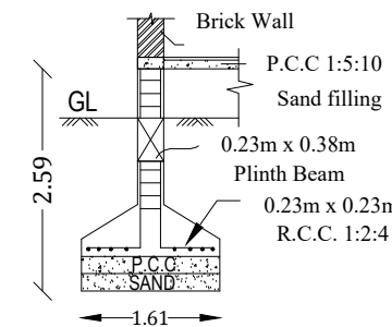
FOUNDATION DETAILS
