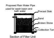
Section of Filter Unit
