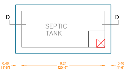
PLAN OF SEPTIC TANK SCALE 1"=2'0"
