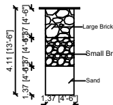
SECTION OF RAIN WATER
