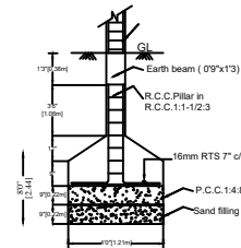
FOUNDATION DETAILS
