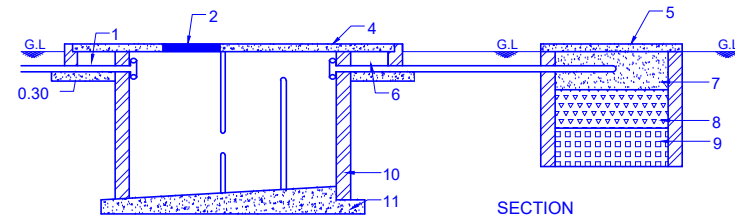
SECTION
