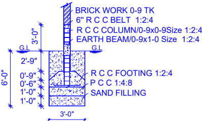
FOUNDATION
