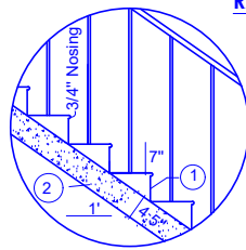
STAIRCASE SECTION
