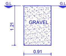
TRIAL PIT
