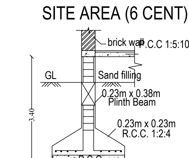
FOUNDATION DETAILS
