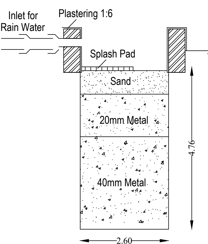
RAIN WATER PERCOLATION PIT
