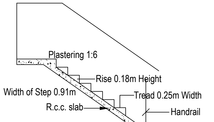
DETAILS OF STAIR CASE
