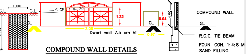
COMPOUND WALL DETAILS
