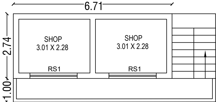
PRO. FIRST FLOOR PLAN
