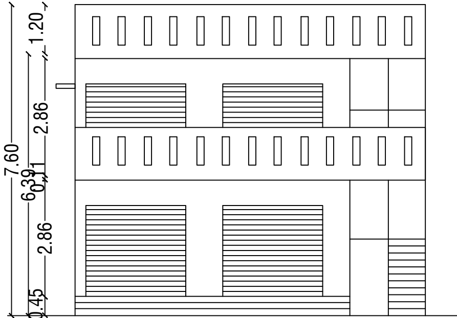
FRONT ELEVATION.
