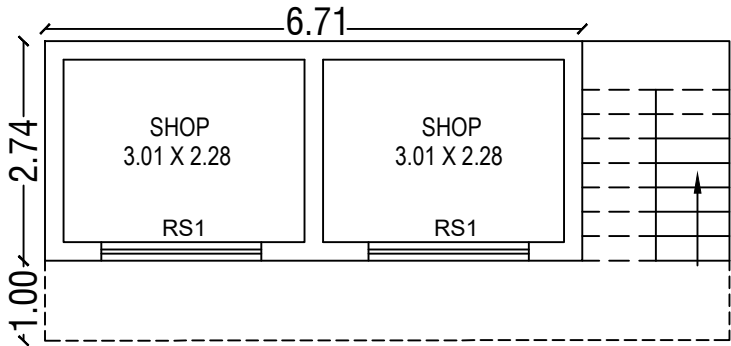
EXTG. GROUND FLOOR PLAN
