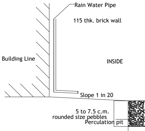
PERCOLATION PIT
