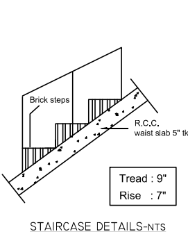
STAIRCASE DETAILS-NTS
