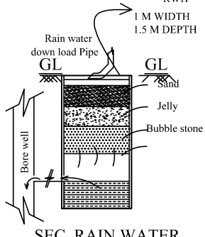
SEC. RAIN WATER HARVEST PIT
