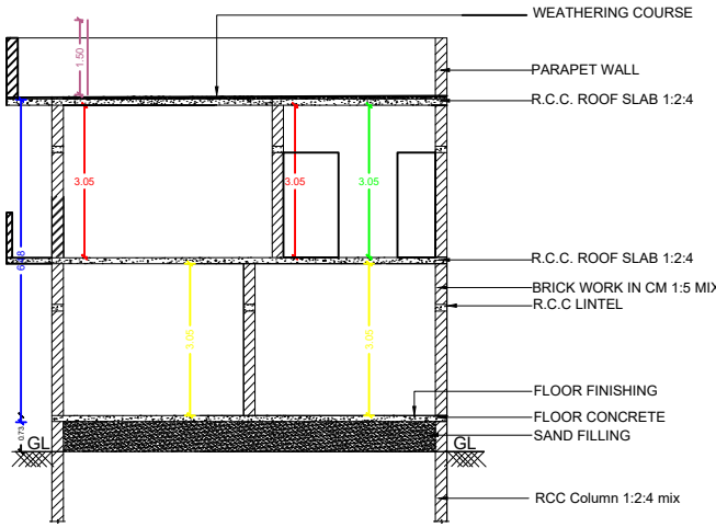
SECTION - 'RI'
