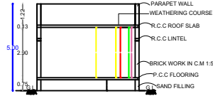
SECTION ON A-A
