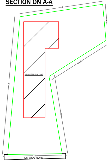
SITE PLAN
