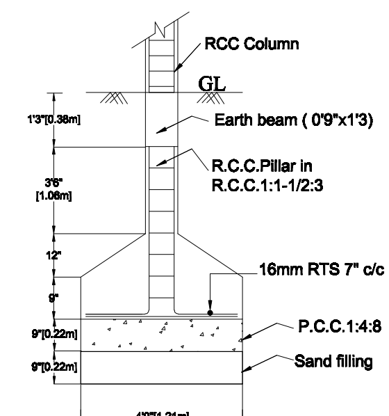
FOUNDATION DETAILS
