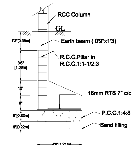
FOUNDATION DETAILS
