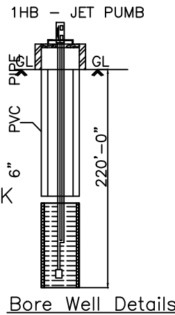
Bore Well Details
