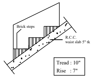
STAIRCASE DETAILS-nts
