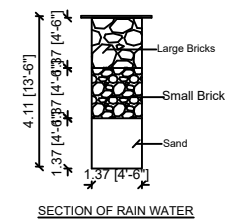
SECTION OF RAIN WATER
