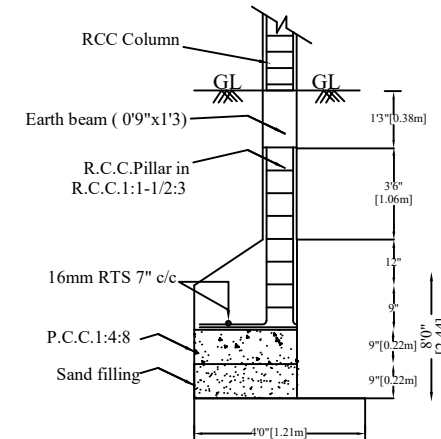
FOUNDATION DETAILS
