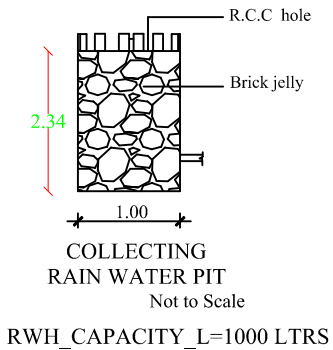
COLLECTING RAIN WATER PIT Not to Scale RWH_CAPACITY_L=1000 LTRS
