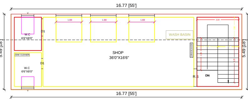
PRO.FIRST FLOOR
