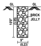
PERCULATION PIT
