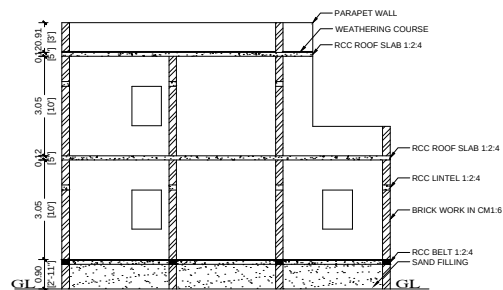
SECTION "A-B"
