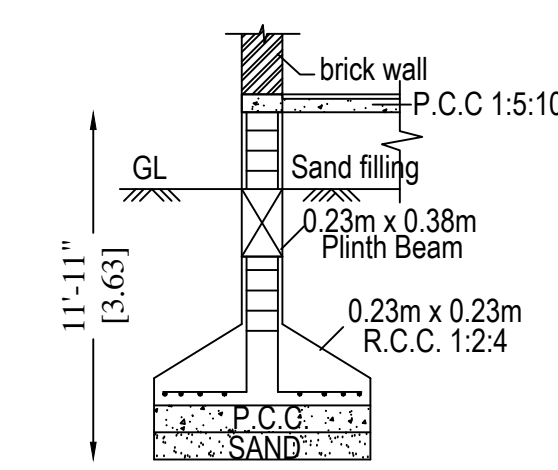
FOUNDATION DETAILS
