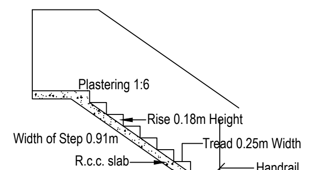
DETAILS OF STAIR CASE
