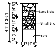
SECTION OF RAIN WATER
