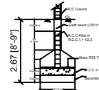
FOUNDATION DETAILS
