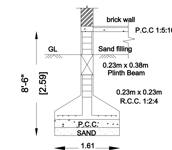
FOUNDATION DETAILS
