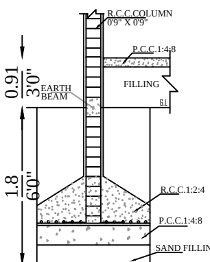
FOUNDATION DETAILS
