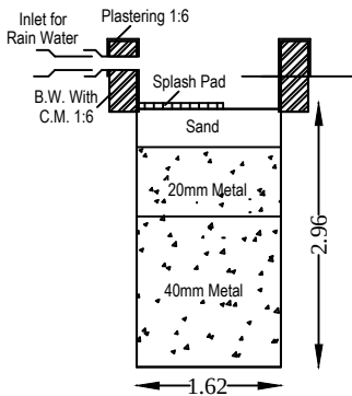
RAIN WATER PERCOLATION PIT
