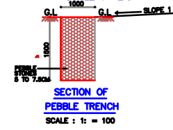
SECTION OF PEBBLE TRENCH
