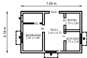
PROPOSED FIRST FLOOR PLAN
