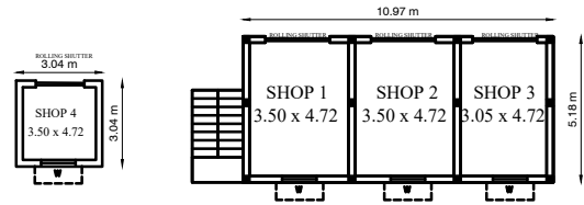
PROPOSED GROUND FLOOR PLAN
