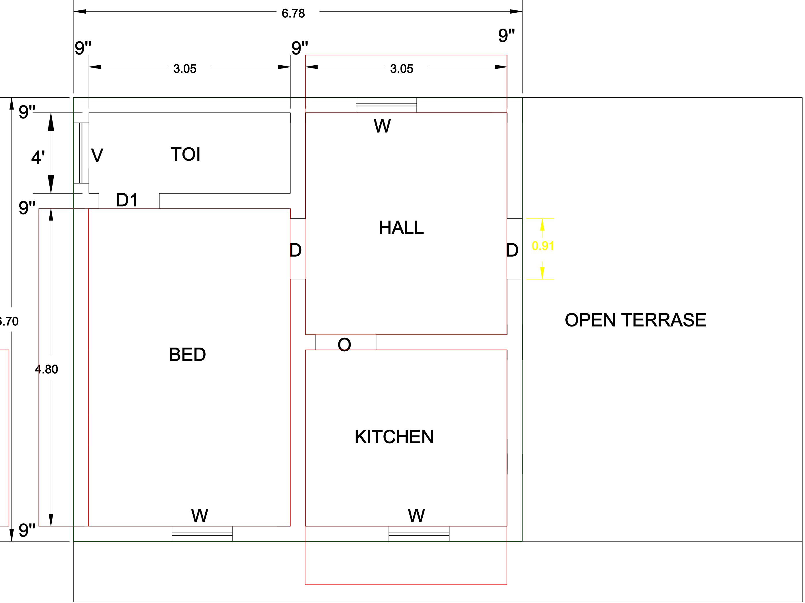
PROSED F.F PLAN
