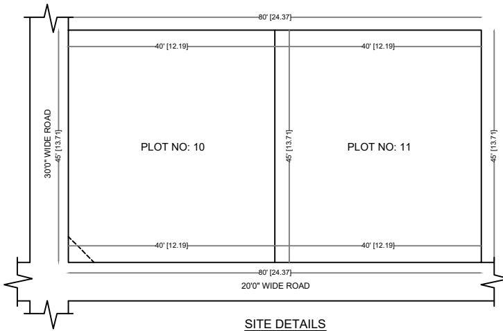
SITE DETAILS
