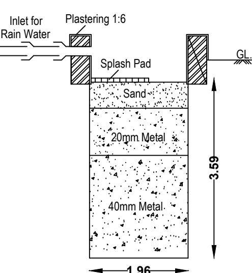
RAIN WATER PERCOLATION PIT
